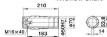
FA77/FAF77/FAZ77空心轴 /Hollow shaft
